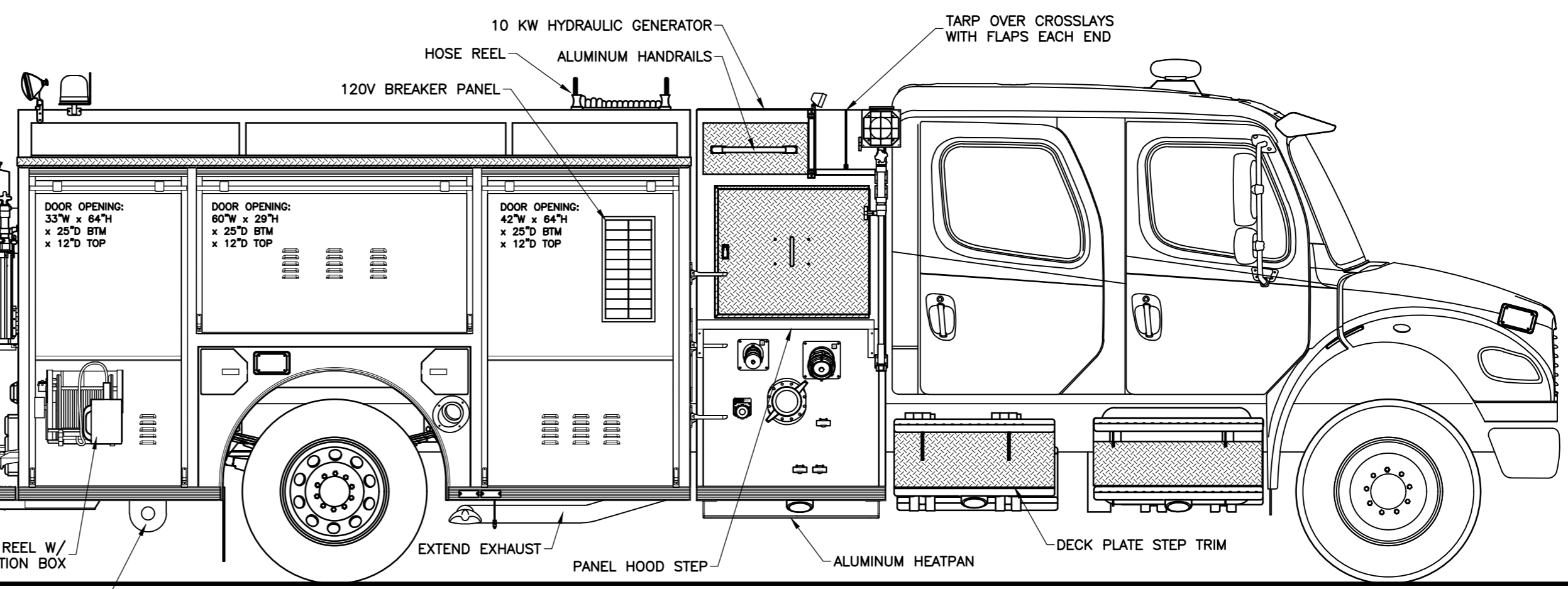
RIGHT SIDE
