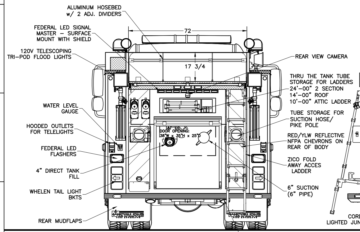
REAR
