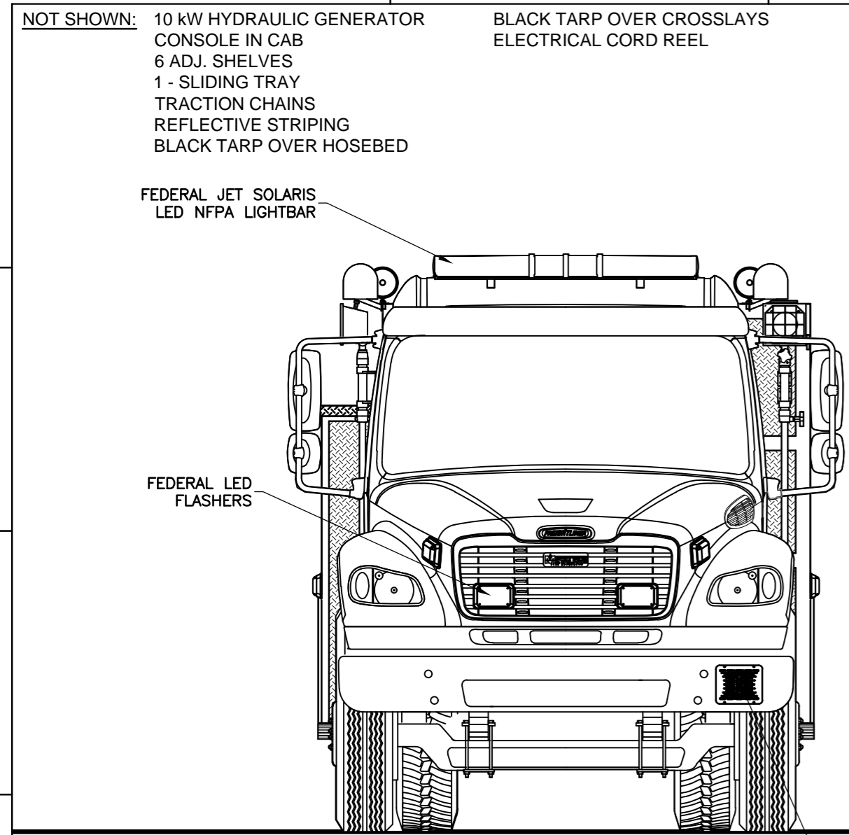
FRONT
